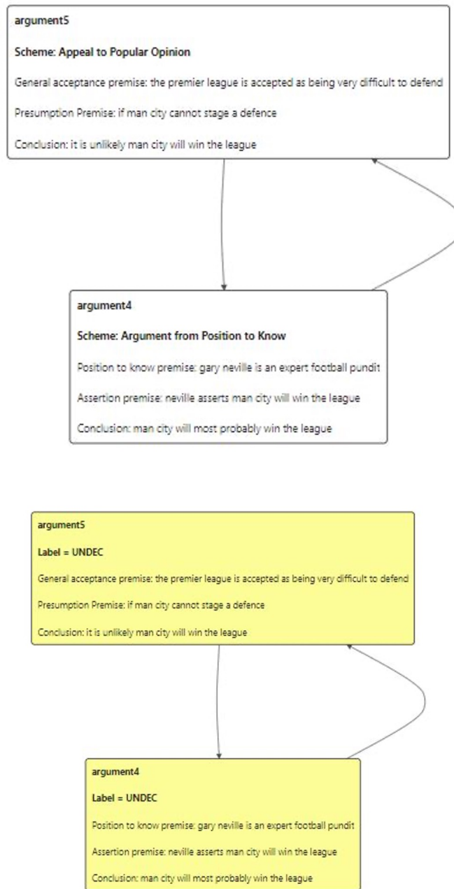
Figure 11.8: An argument graph created by users during formal UX testing with conflicting claims considering whether Man City will win the Premier League in 2021/2. Both arguments are UNDEC under the grounded labelling [8].
