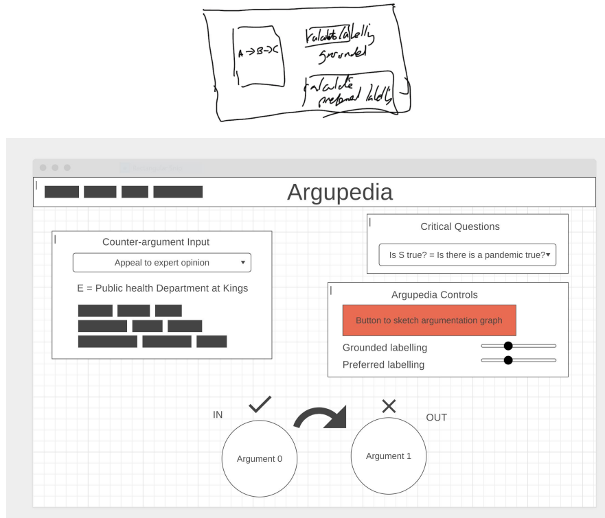
Figure 6.4: Professor Modgil sketch of application in black (above) with prototype built (below) demonstrating switches to add to the argument graph labelling algorithms.
