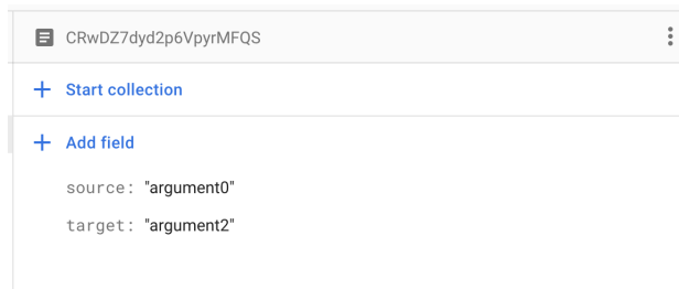
Figure 9.2: The links between arguments were stored in another Firestore collection separately and simply store links between argument IDs.
