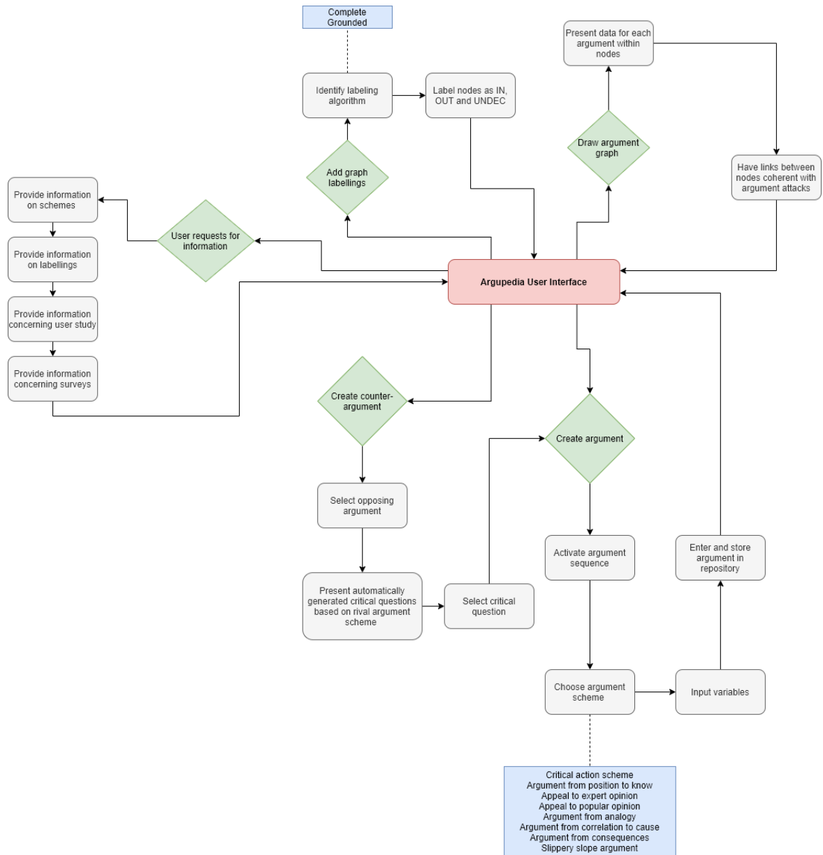
Figure 6.8: An Argupedia state diagram of all the possible stages and changes of the interface for the user.
