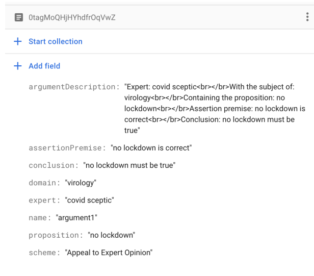
Figure 9.1: Data encapsulated in single argument submission including the argument name (ID), argument scheme, argument description and user provided variables.
