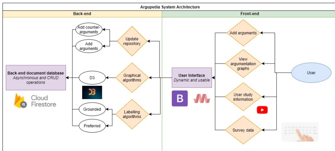
Figure 6.7: An envisaged architecture diagram for Argupedia to operate.
