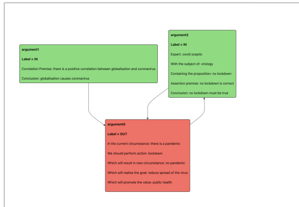
Figure 11.6: Arguments denoted in green (IN) and red (OUT) under the grounded labelling.
